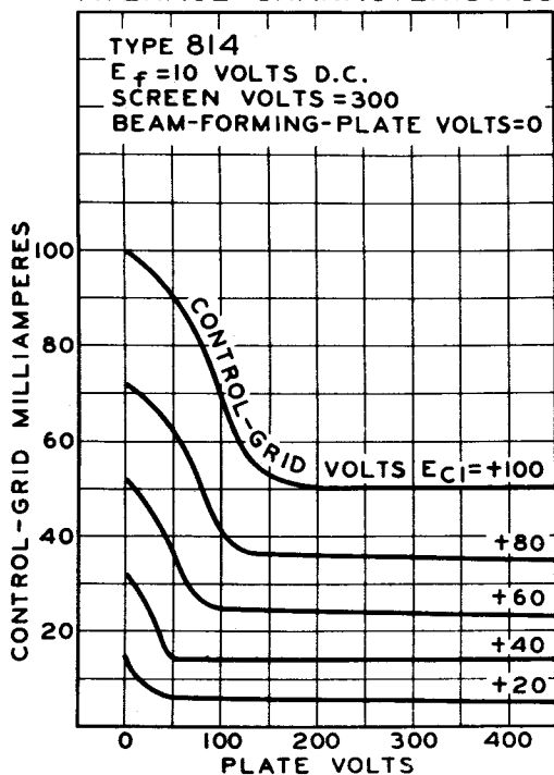
AVERAGE CHARACTERISTICS
