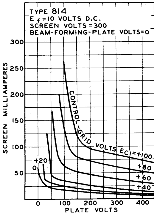
AVERAGE CHARACTERISTICS
